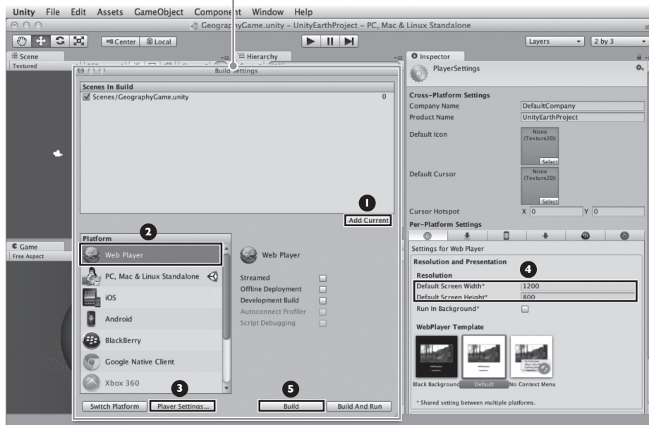
Build Settings window
